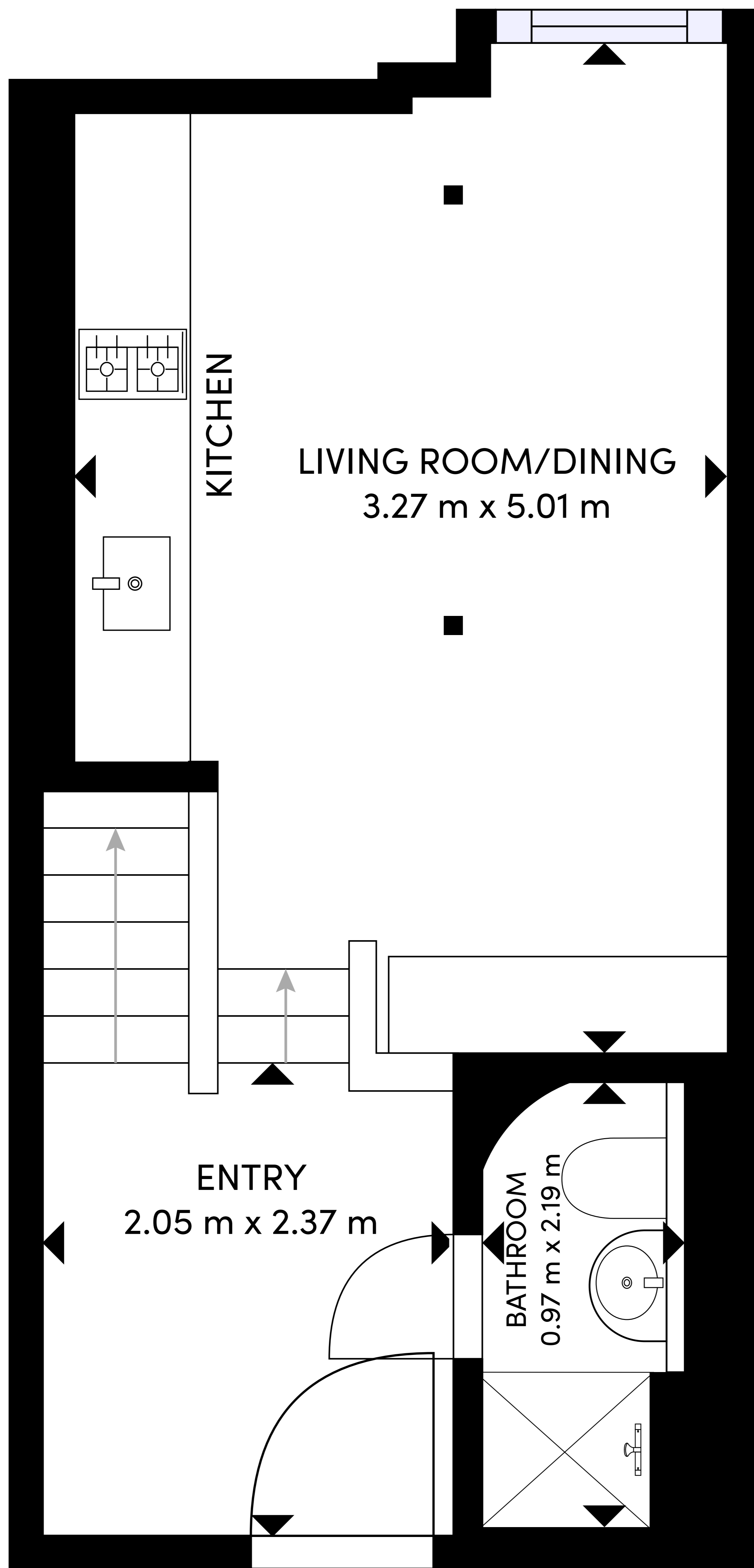
GROUND FLOOR
